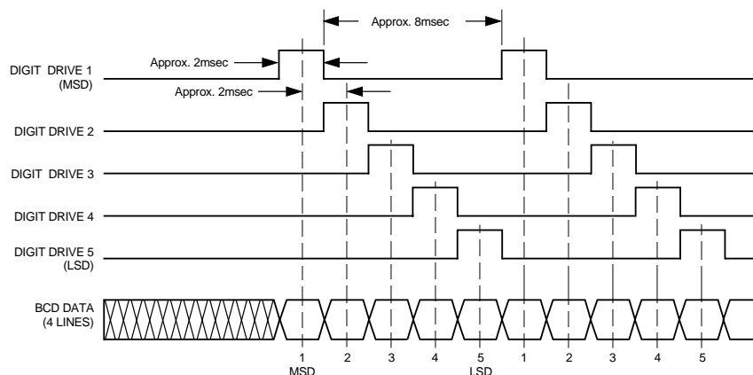
Figure 2. BCD Data Timing Diagram
