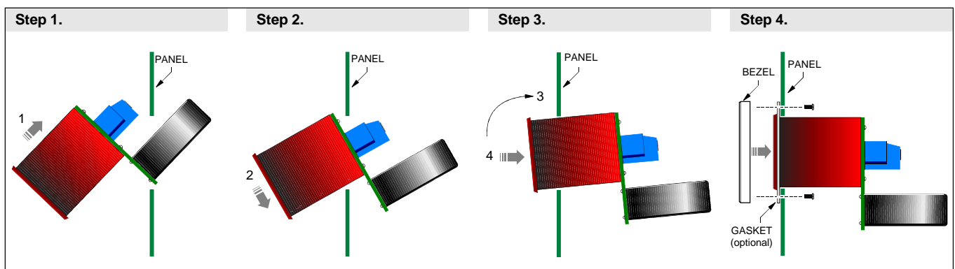
Figure 2. Panel Installation
