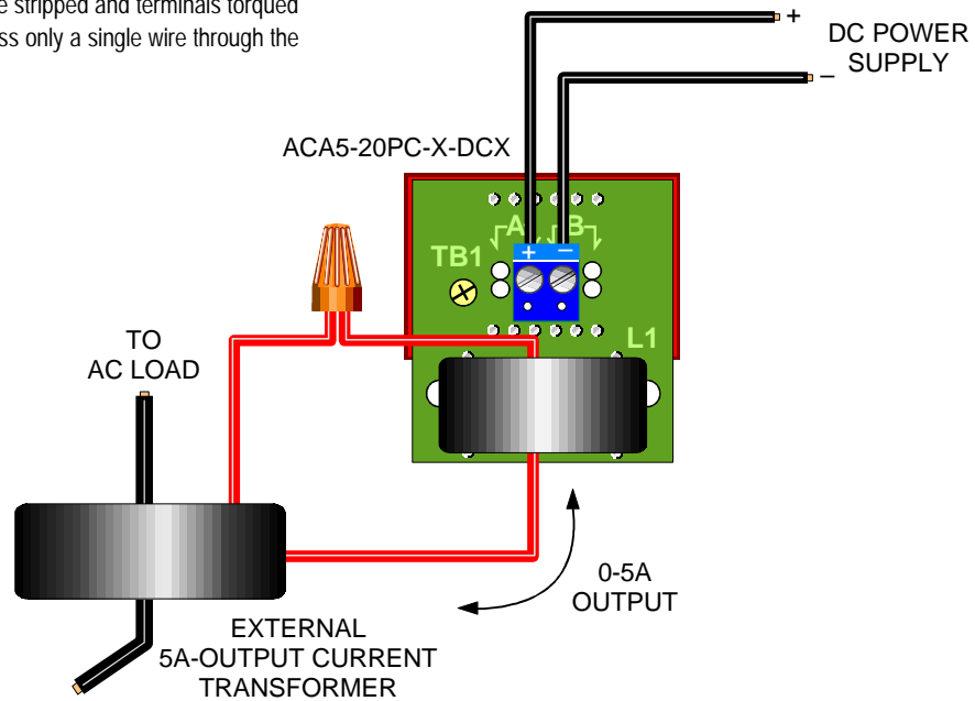
Figure 4. All ACA5-20PC DC-Powered Models
