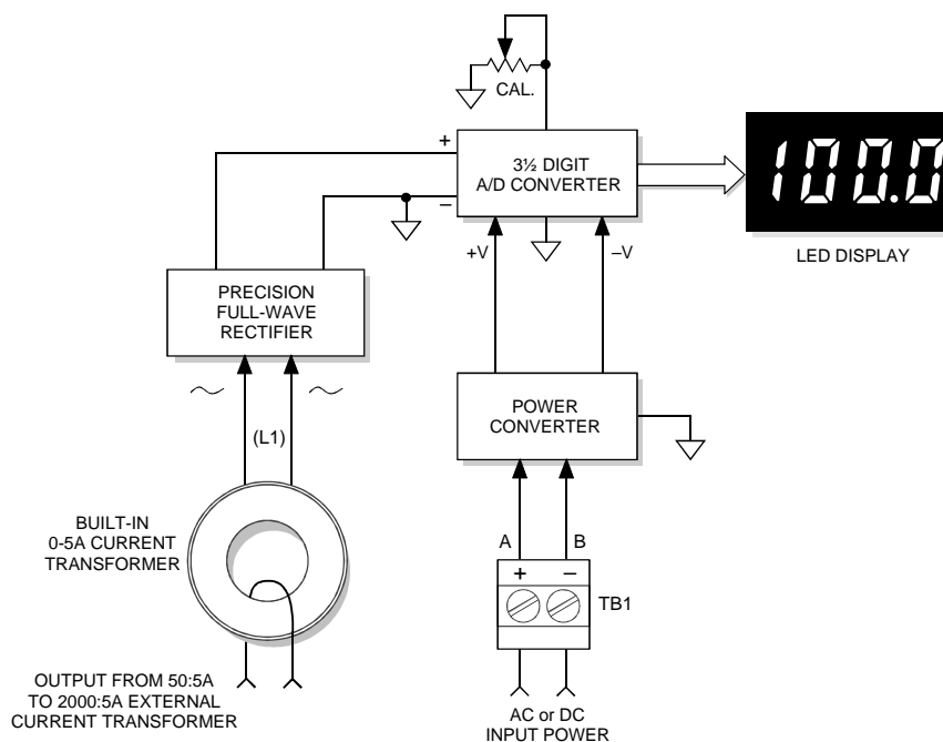
Figure 1. ACA5-20PC Series Simplified Schematic
