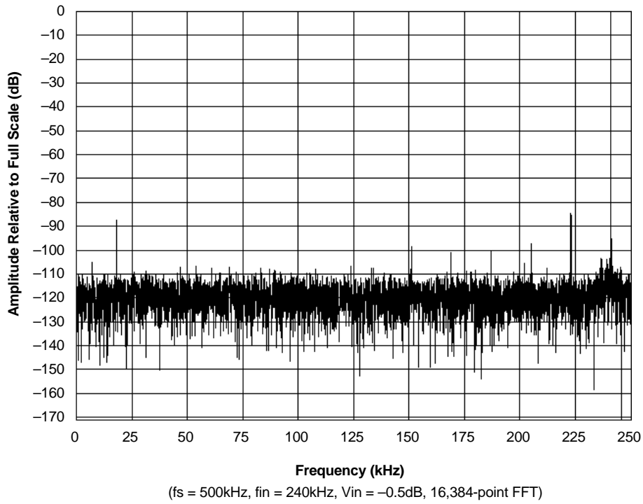
Figure 6. ADS-916 FFT Analysis
