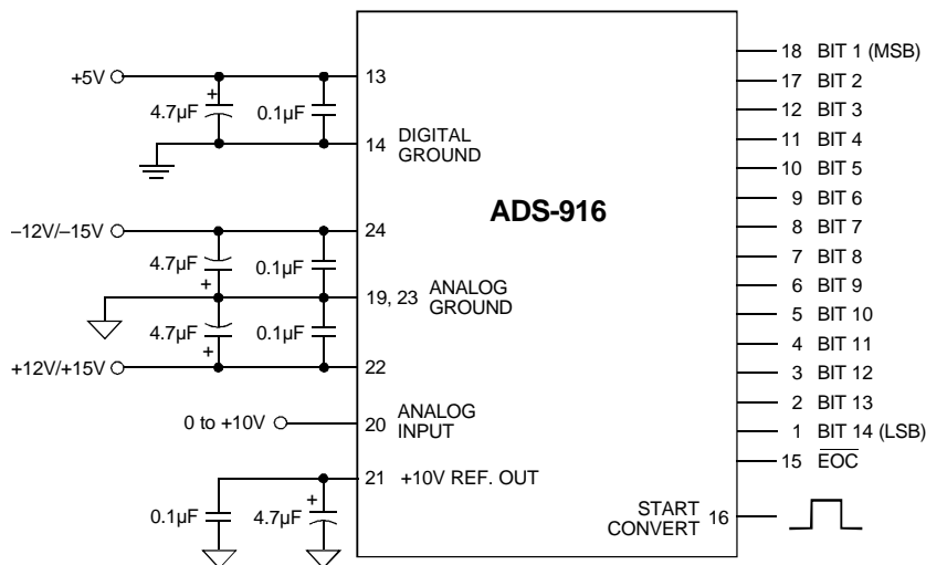
Figure 3. Typical ADS-916 Connection Diagram
