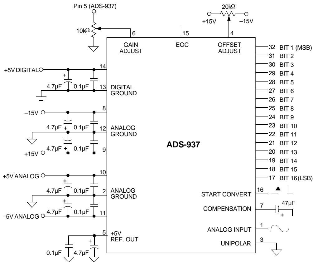
Figure 2. Typical ADS-937 Connection Diagram
