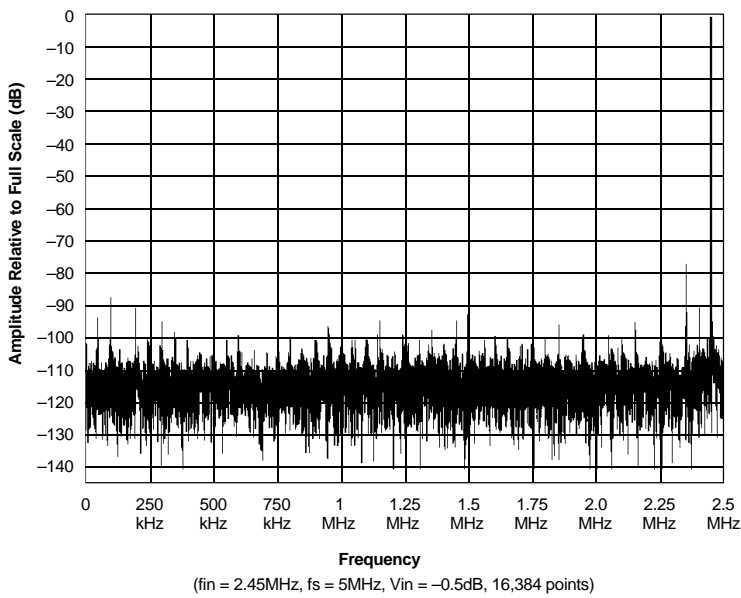
Figure 5. ADS-944 FFT
