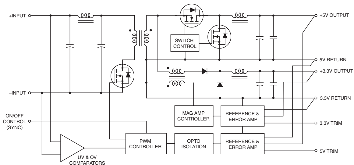
Figure 1. Simplified Schematic
