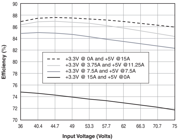
Overall Efficiency vs. Line and Load
