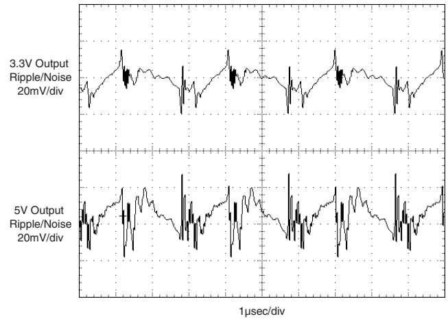
Output Ripple and Noise (PARD) (VIN = 48V, 5V@7.5A, 3.3V @ 7.5A, external 10µF || 1µF output capacitors.)
