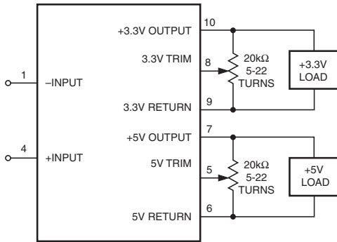
Figure 3A. Trim Connections Using a Trimpot
