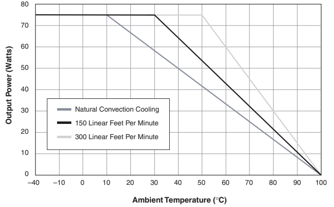
Output Power vs. Ambient Temperature (With HS-CP heat sink, 5V Output, 3.3V @ 0A.)
