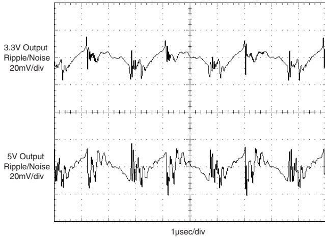
Output Ripple and Noise (PARD) (VIN = 24V, 5V@7.5A, 3.3V @ 7.5A, external 10µF || 1µF output capacitors.)
