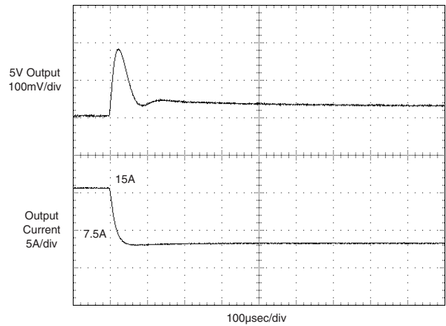
5V Output Full-Load to Half-Load Transient Response (VIN = 48V, 3.3V@ 0A, external 10µF || 1µF output capacitors.)
