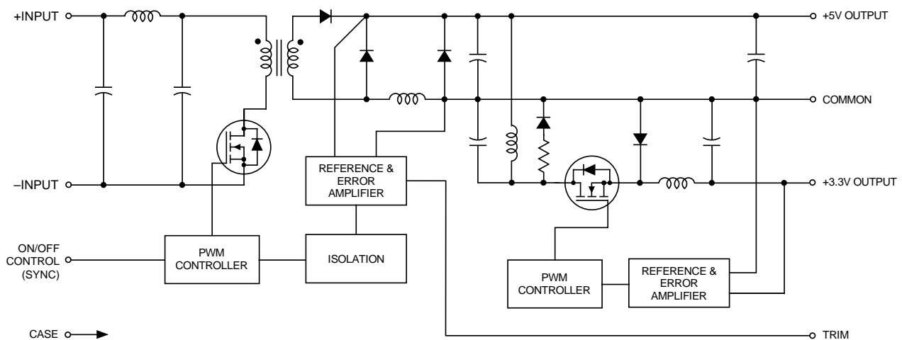
Figure 1. Simplified Schematic
