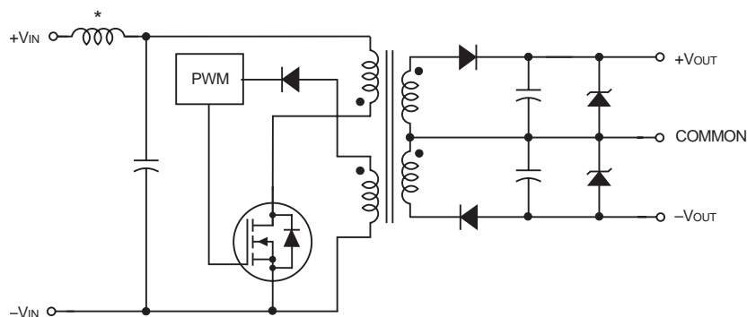
Figure 1. Simplified Schematic
