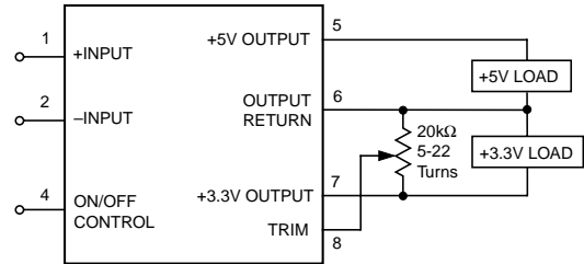
Figure 3. Trim Connections using a Trimpot
