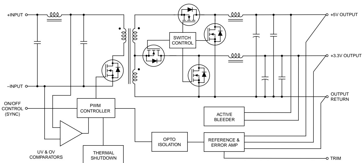
Figure 1. Simplified Schematic
