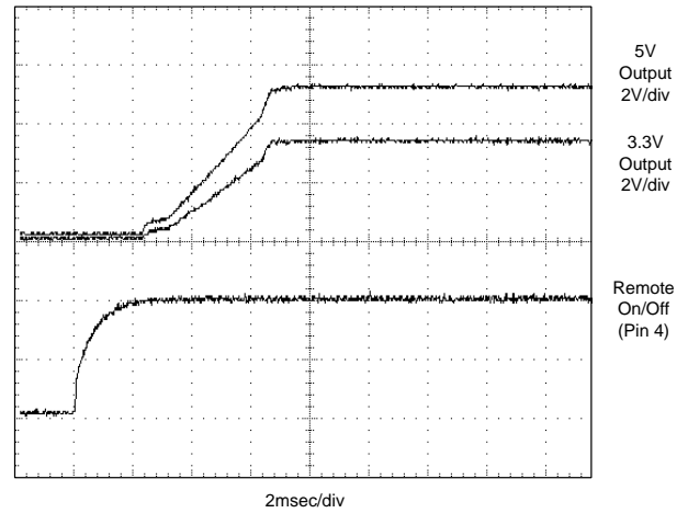
Start-Up from Remote On/Off Control ( V_{IN} = nominal, 5V @ 3A, 3.3V @ 4.5A, external 1 \mu F output capacitors.)
