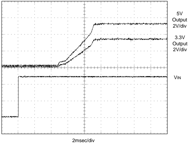
Start-Up from V_{IN} ( V_{IN} = nominal, 5V @ 3A, 3.3V @ 4.5A, external 1 \mu F output capacitors.)
