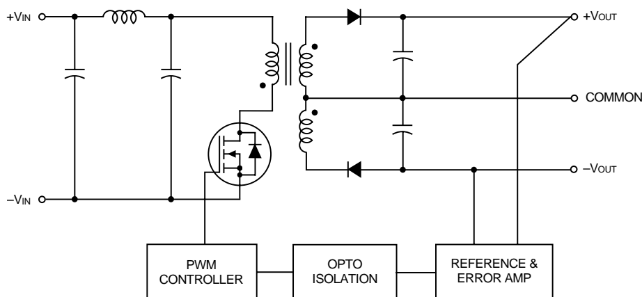
Figure 1. Simplified Schematic
