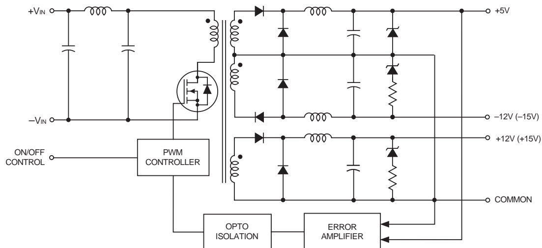
Figure 1. Simplified Schematic
