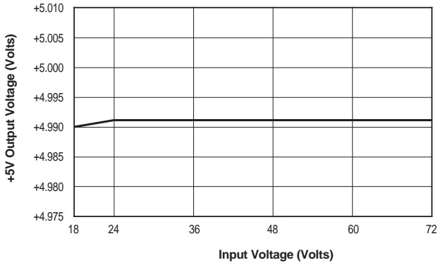
+12V Line Regulation (+5V output loaded @ 2.75A, ±12V outputs loaded @ ±250mA)
