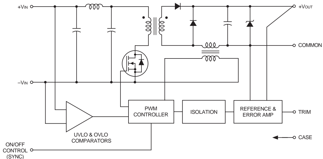
Figure 1. Simplified Schematic
