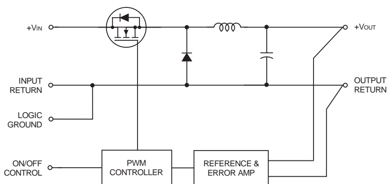
Figure 1. Simplified Schematic
