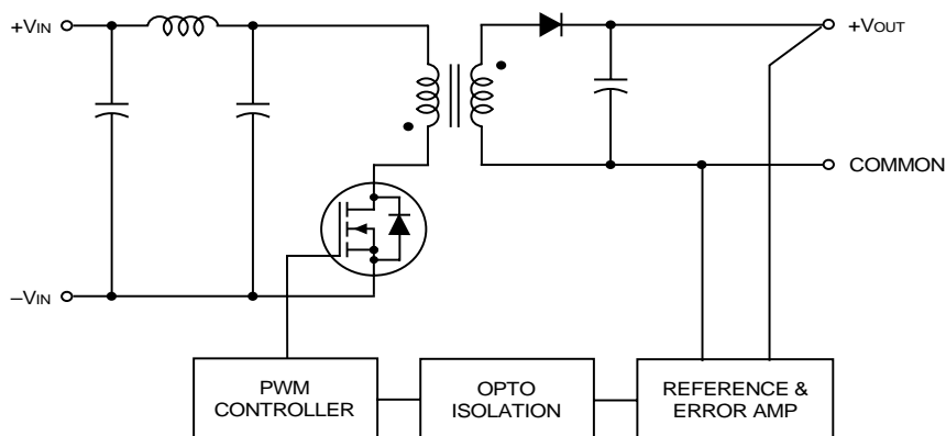
Figure 1. Simplified Schematic
