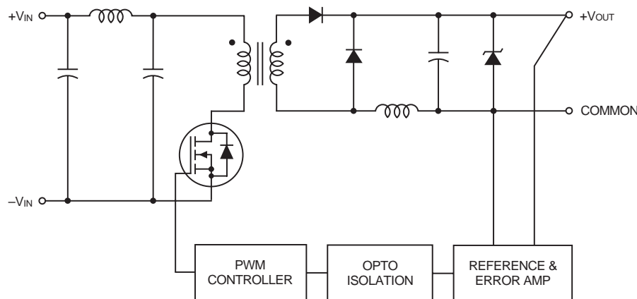
Figure 1. Simplified Schematic
