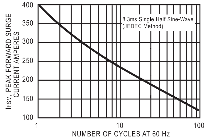
FIG. 6 - MAXIMUM NON-REPETITIVE FORWARD SURGE CURRENT UNIDIRECTIONAL
