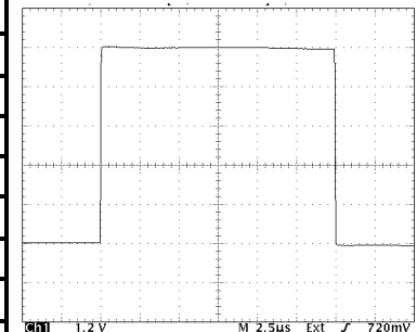
Typical Output Waveform, 6000V Output (2.5µs/Div horizontal scale, 1.2kV/Div vertical scale)
