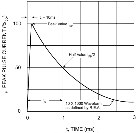
Fig. 1 Pulse Waveform
