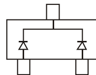
BAV170T Marking: 51
