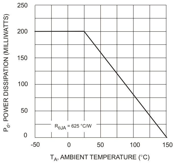
Fig. 1 Derating Curve
