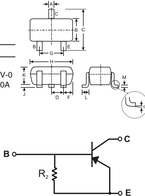
SCHMATIC DIAGRAM
