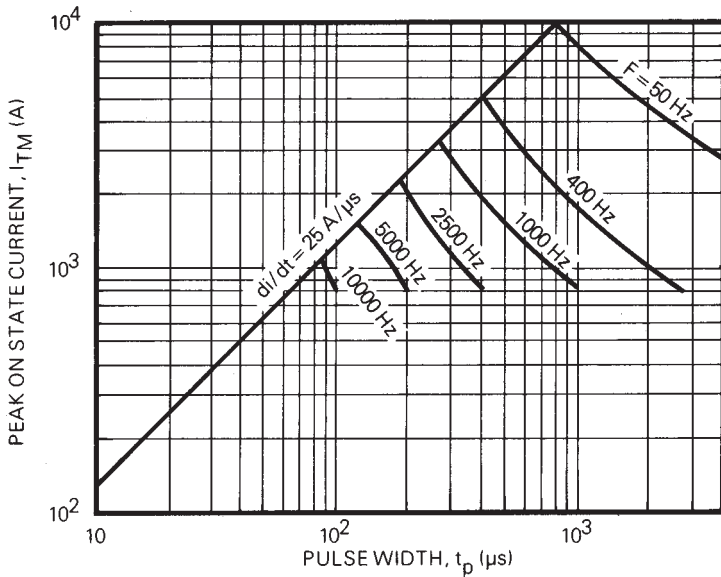
FIG.10 MAXIMUM ALLOWABLE PEAK ON-STATE CURRENT vs PULSE WIDTH FOR T_c = 65^\circ C
