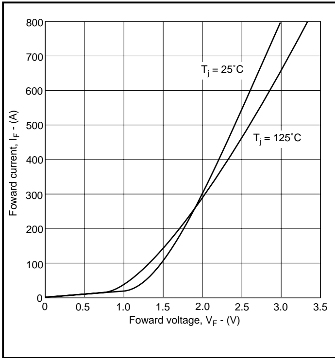
Fig. 10 Diode typical forward characteristics
