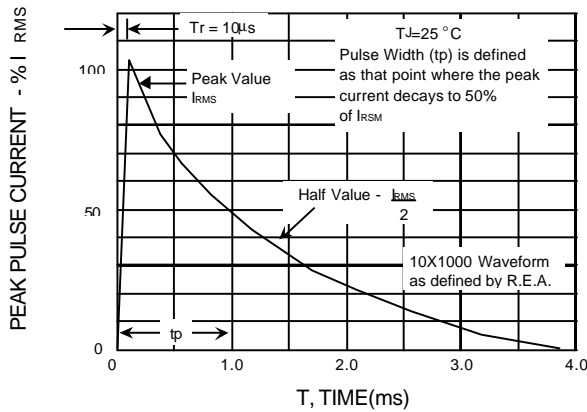
FIG.5 - PULSE WAVEFORM
