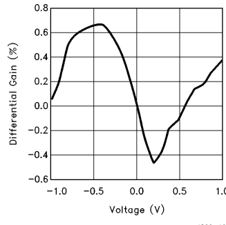
Differential Gain at V_S = \pm 5V
