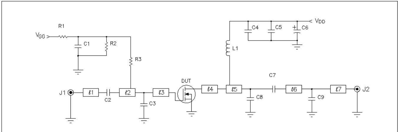
Test Circuit Schematic for f = 960 MHz
