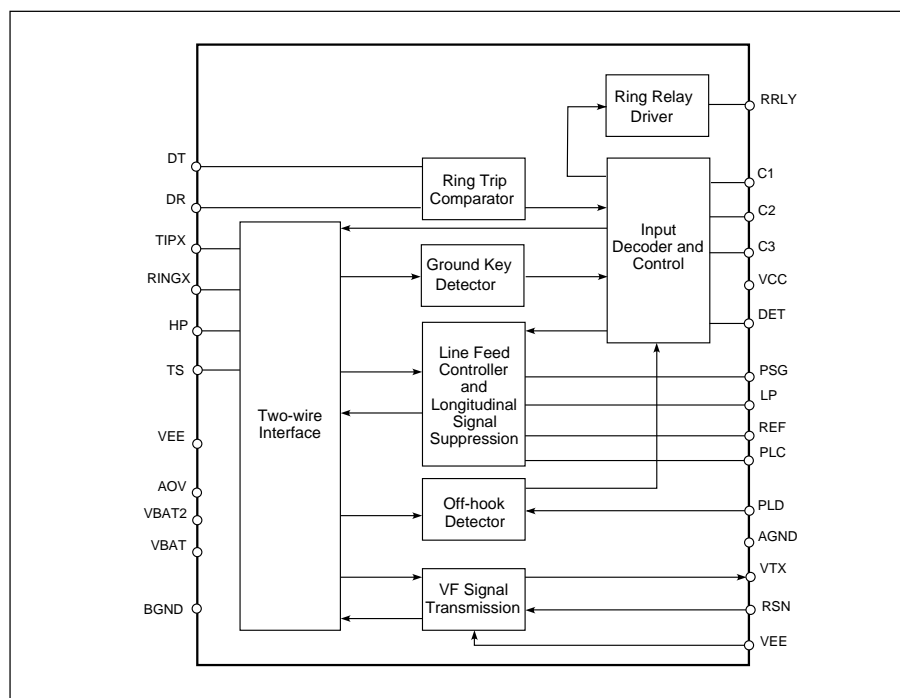
Figure 1. Block diagram.
