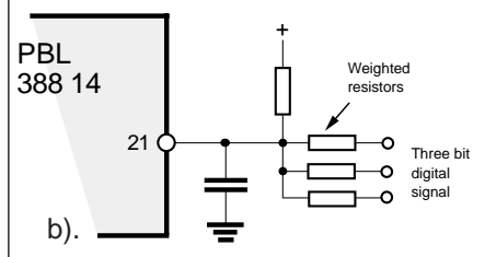
Figure 17. DC - volume control options.
