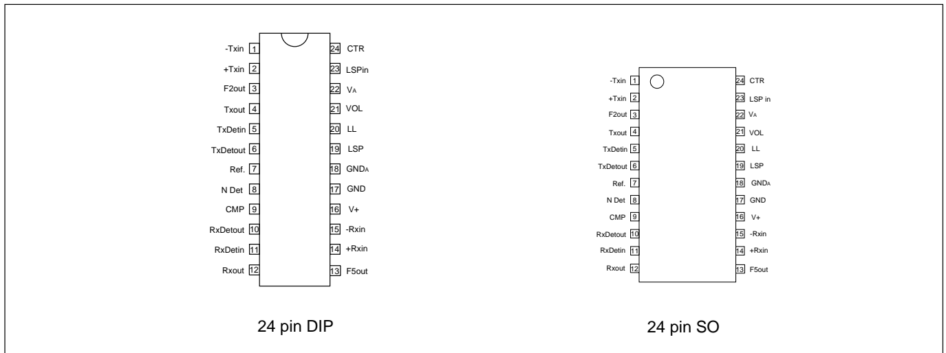
Figure 4. Pin configuration.
