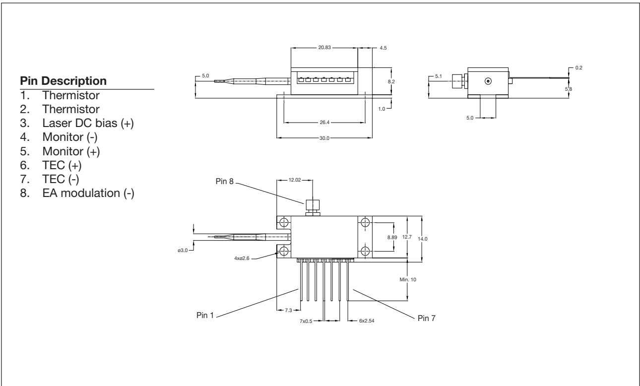
Figure 2. Pin description
