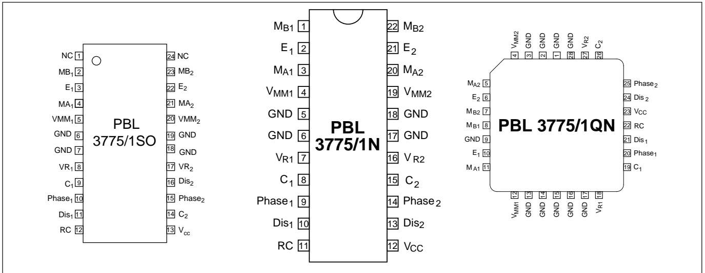
Figure 4. Pin configuration.
