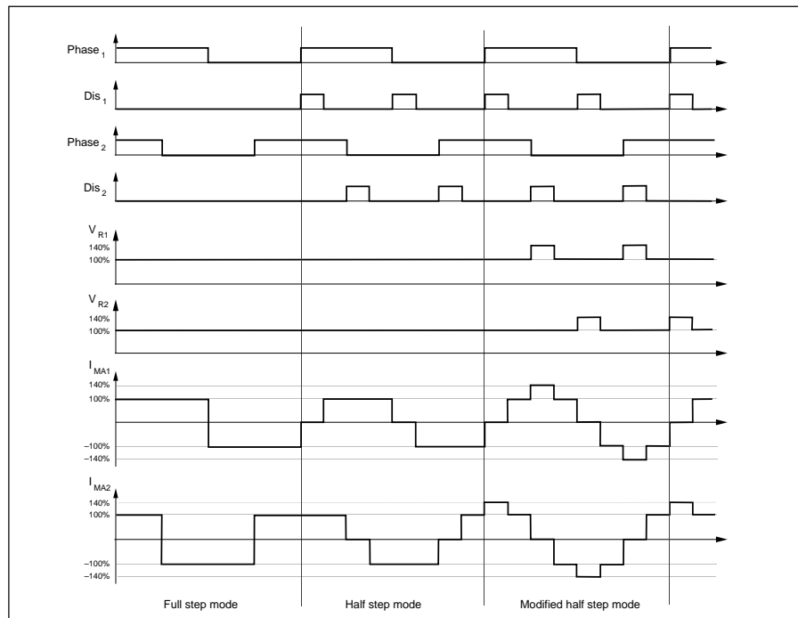
Figure 15. Stepping modes.
