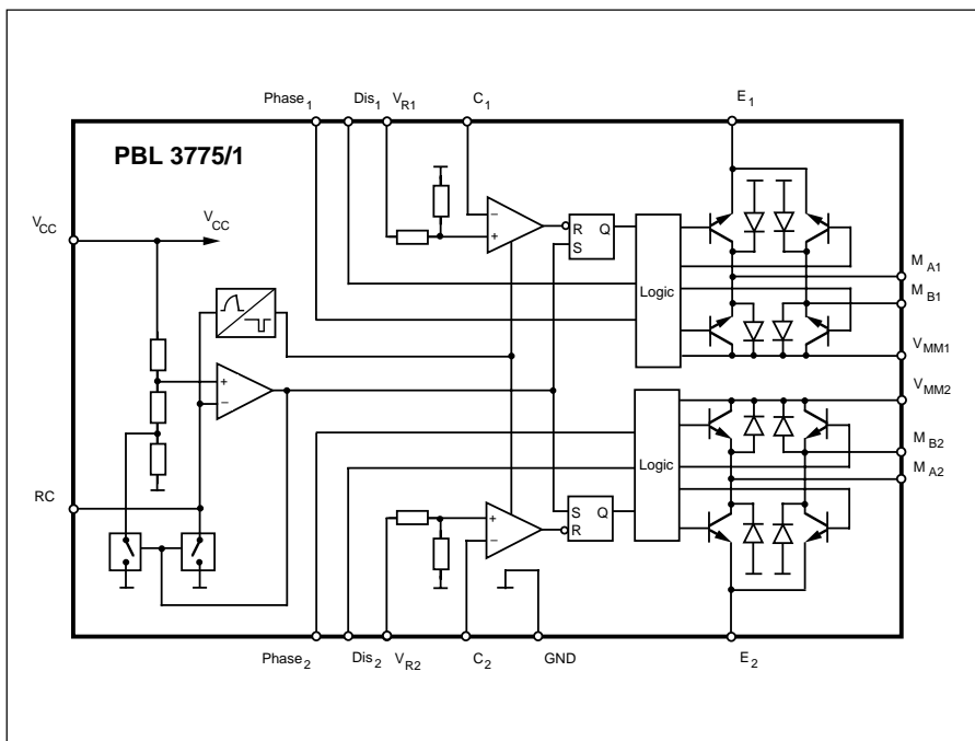
Figure 1. Block diagram
