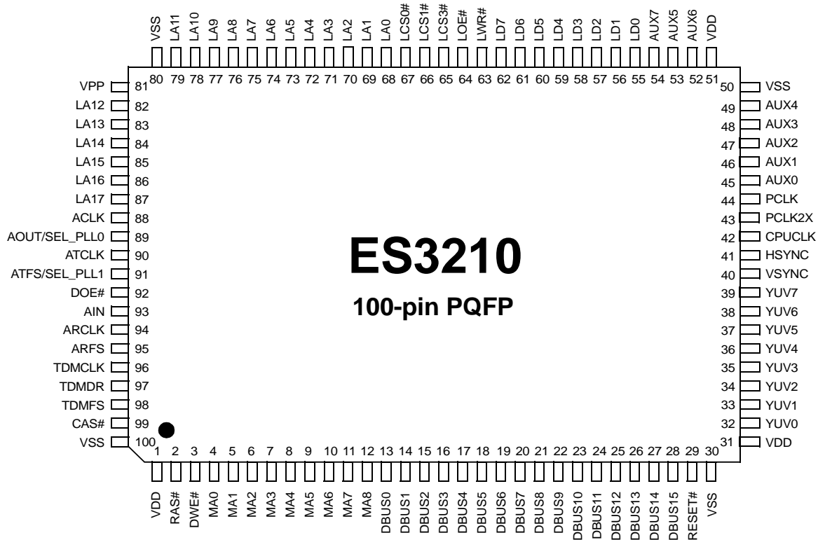
Figure 1 ES3210 Pinout Diagram
