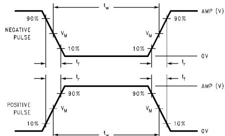
FIGURE 2. V_M = 1.5V
