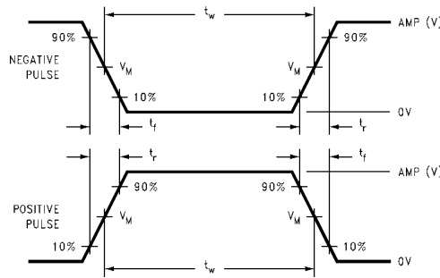
FIGURE 2. V_M = 1.5\text{V}
