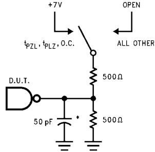
FIGURE 15. Standard AC Test Load
