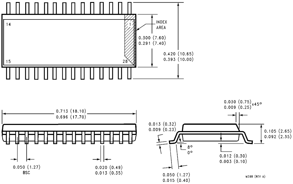
28-Lead Small Outline Integrated Circuit (SOIC), MS-013, 0.300" Wide Body Package Number M28B
