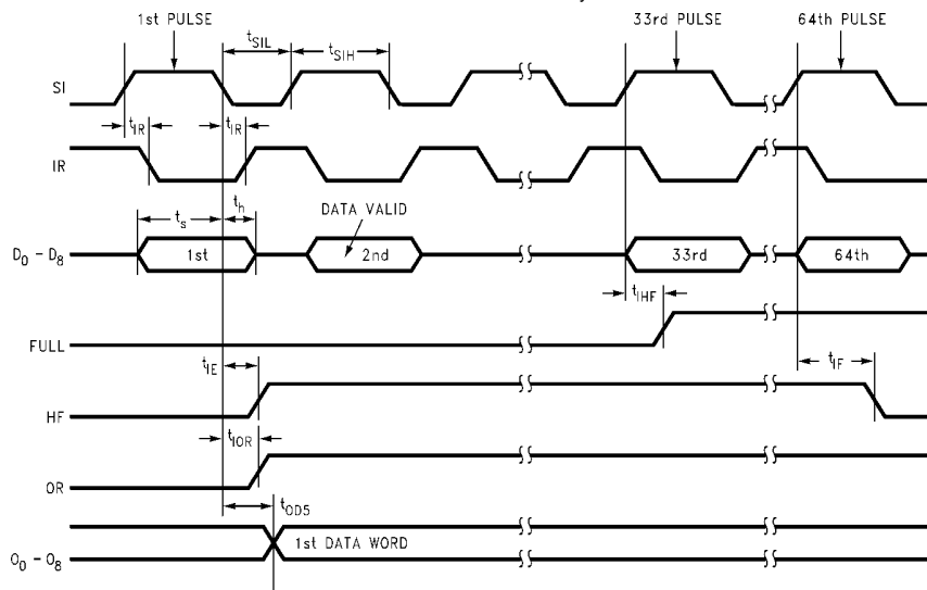
FIGURE 1. Modes of Operation Mode 1
