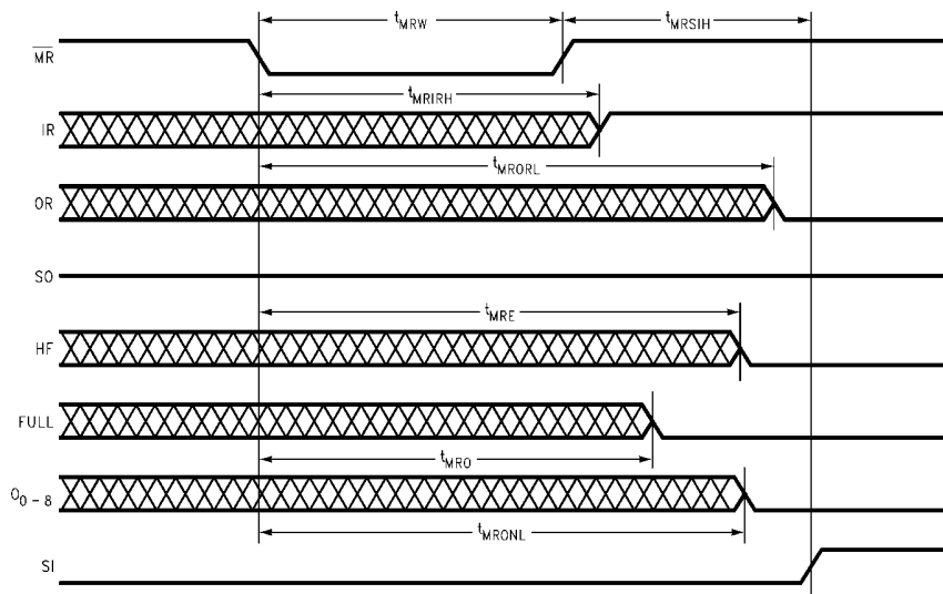
FIGURE 2. Mode of Operation Mode 2
