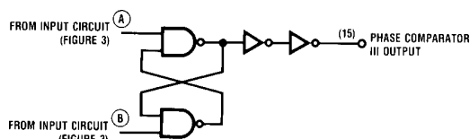
FIGURE 7. Phase Comparator III Logic Diagram
