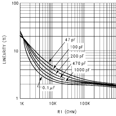
VCO WITHOUT OFFSET R 2 = ∞
