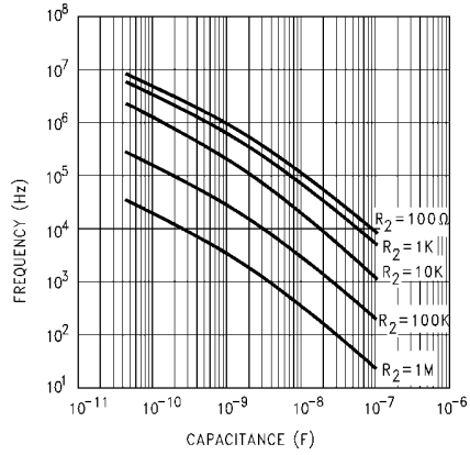
Typical Offset Frequency vs R_2, C_1 V_{CC} = 4.5V T = 25^\circ C V_{COIN} = GND R_1 = OPEN
