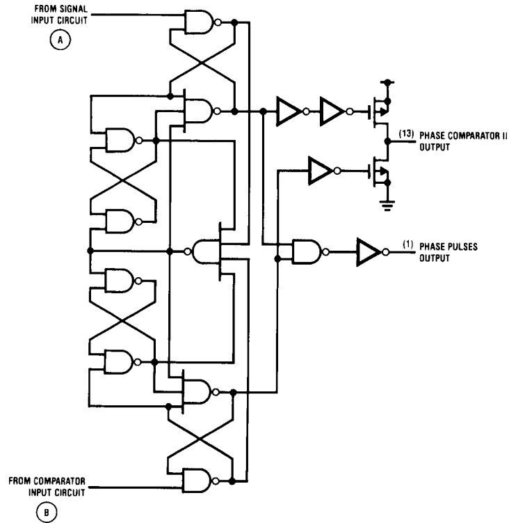
FIGURE 5. Logic Diagram for Phase Comparator II
