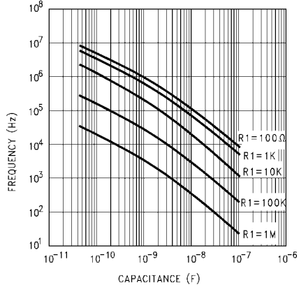
Typical Center Frequency vs R_1, C_1 V_{CC} = 4.5V V_{COIN} = V_{CC}/2 R_2 = OPEN
