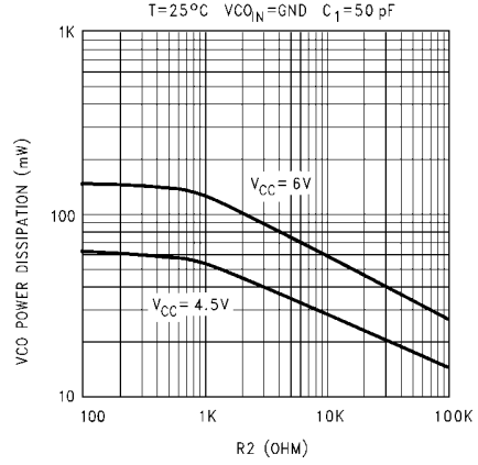
VHC4046 Typical VCO Power Dissipation @ f_{MIN} vs R_2
