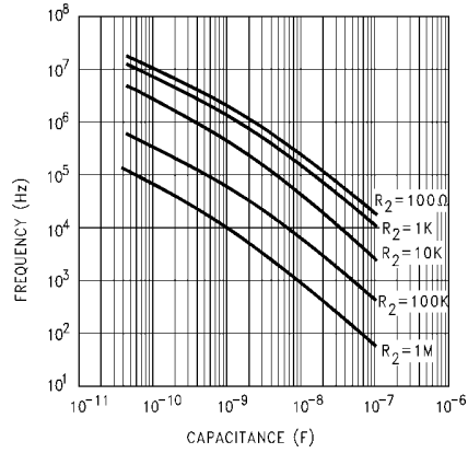
Typical Offset Frequency vs R_2, C_1 V_{CC} = 6V T = 25^\circ C V_{COIN} = GND R_1 = OPEN
