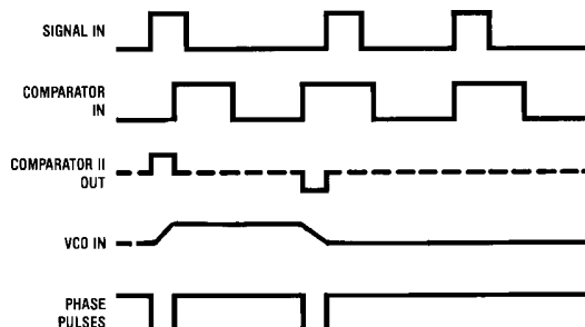
FIGURE 6. Typical Phase Comparator II Output Waveforms
