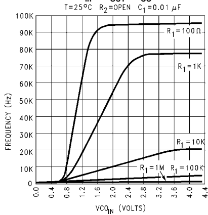
VHC4046 V_{COIN} vs f_{OUT} V_{CC}=4.5\text{V}
