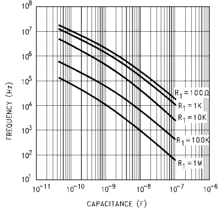
Typical Center Frequency vs R_1, C_1 V_{CC} = 6V V_{COIN} = V_{CC}/2 R_2 = OPEN
