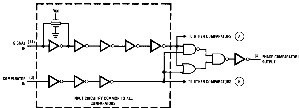
FIGURE 2. Logic Diagram for Phase Comparator I and the Common Input Circuit for All Three Comparators
