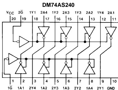
DM74AS240
