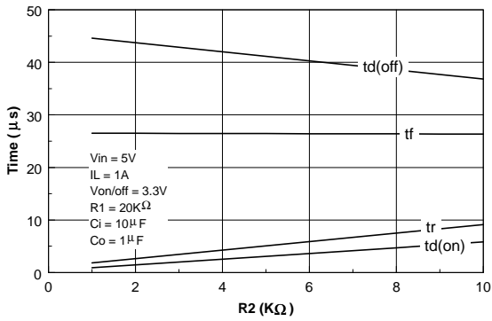
Figure 6. Switching Variation with R2 at Vin = 5V and R1 = 20KOhm.
