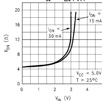
FST3384 V IN vs R ON (Typ)
