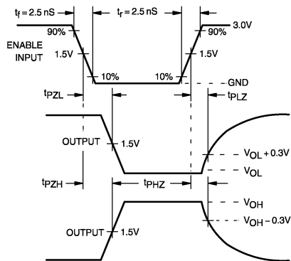
FIGURE 2. AC Waveforms
