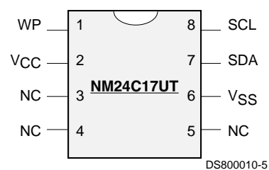
8-Pin TSSOP Package (MT8) Rotated Die (24C17UT)
