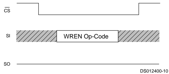
FIGURE 8. Write Enable
