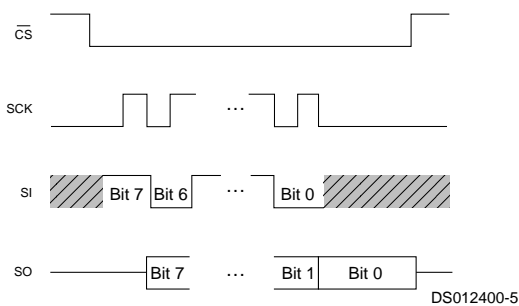
FIGURE 4. SPI Protocol
