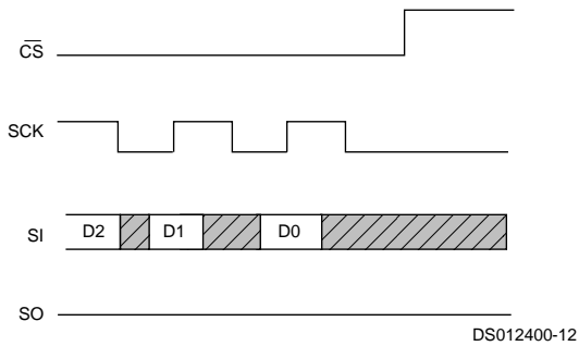
FIGURE 10. Write Sequence
