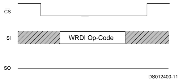
FIGURE 9. Write Disable
