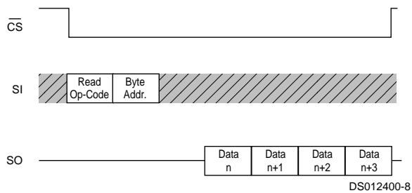
FIGURE 6. Read Sequence
