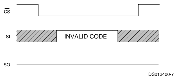
FIGURE 5. Invalid Op-Code
