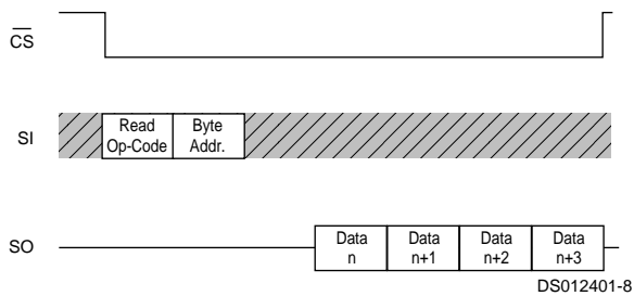
FIGURE 6. Read Sequence
