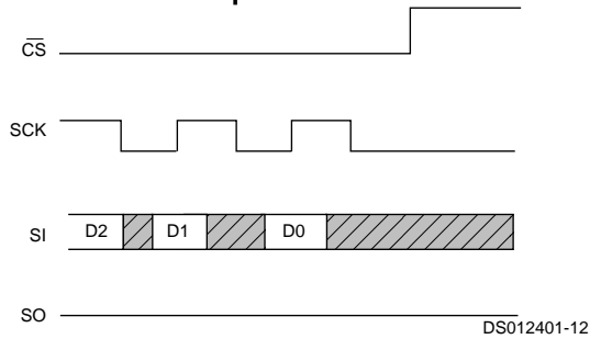
FIGURE 10. Write Sequence
