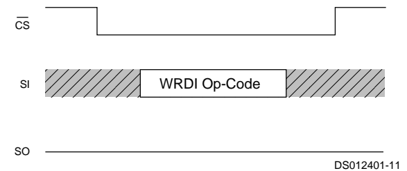
FIGURE 9. Write Disable
