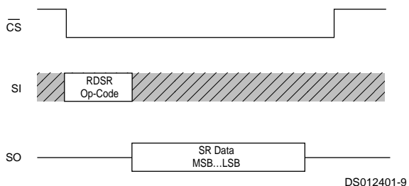
FIGURE 7. Read Status
