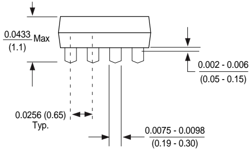
DETAIL A Typ. Scale: 40X
