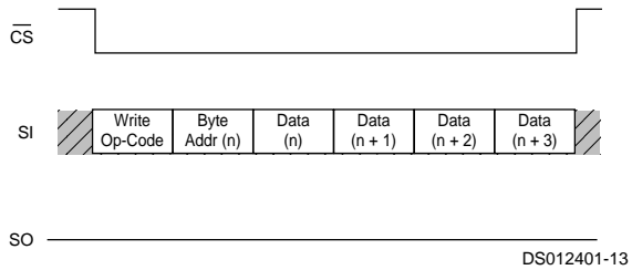
FIGURE 11. 4 Byte Page Write
