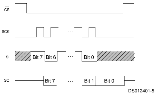
FIGURE 4. SPI Protocol
