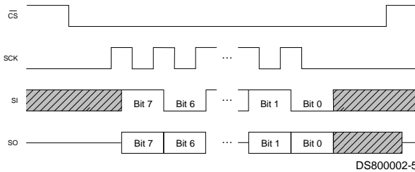
FIGURE 3. SPI Protocol
