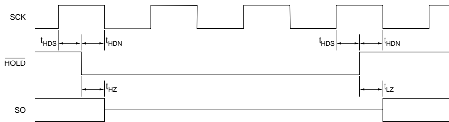
FIGURE 2. HOLD Timing
