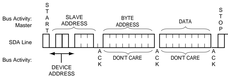
WP Register Write (Figure 7).
