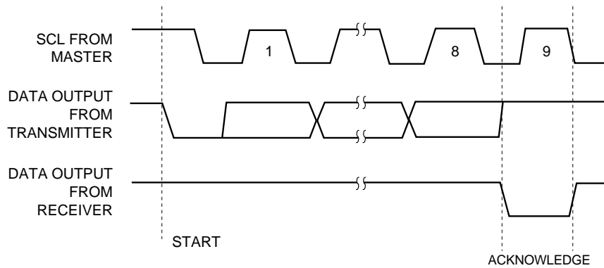
Acknowledge Responses from Receiver (Figure 3).
