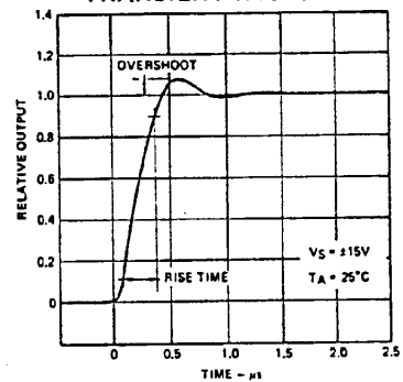
TRANSIENT RESPONSE
