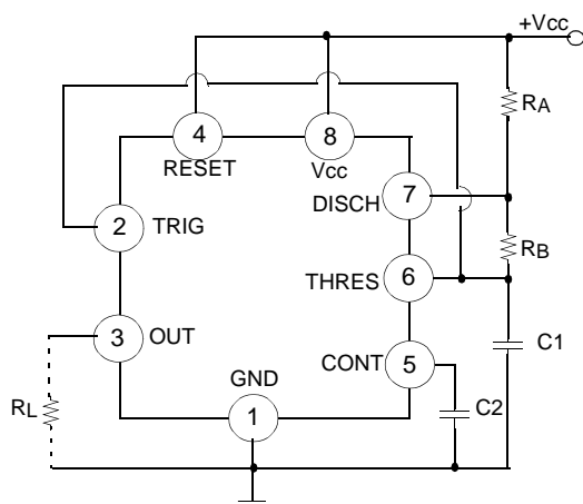
Figure 5. Astable Circuit
