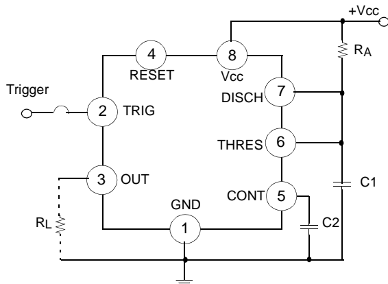
Figure 1. Monoatable Circuit
