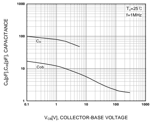
Figure 4. Capacitance
