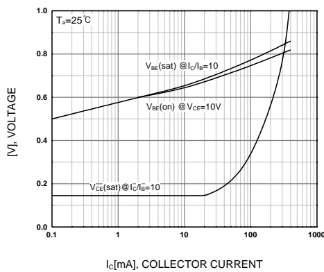
Figure 5. On Voltage
