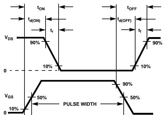
Figure 21. Switching Time Waveforms
