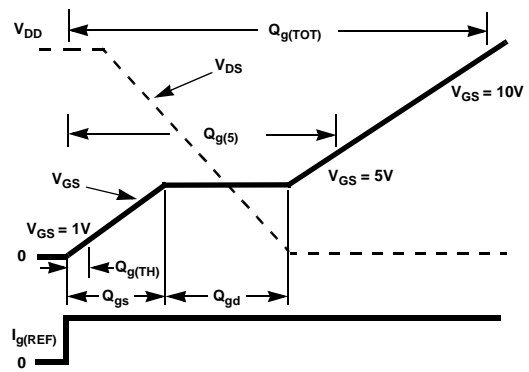
Figure 19. Gate Charge Waveforms
