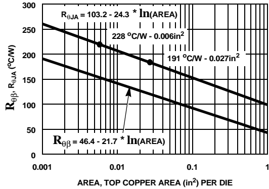
Figure 22. Thermal Resistance vs Mounting Pad Area
