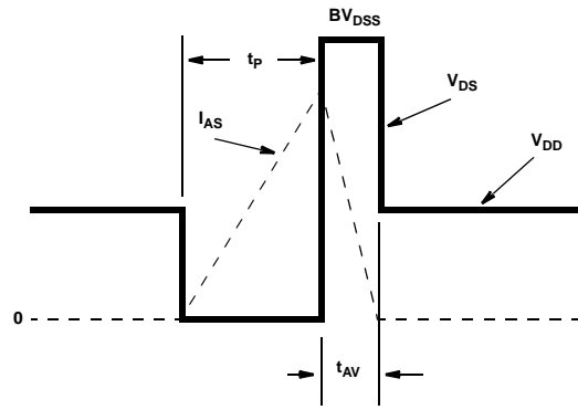
Figure 17. Unclamped Energy Waveforms
