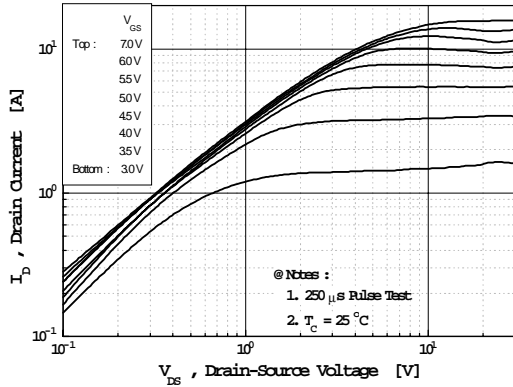
Fig 1. Output Characteristics
