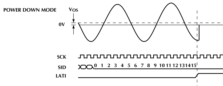
Figure 5. Power Down Mode Waveforms.
